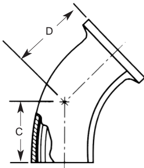
L2KM7 Elbow - Weld x Clamp Standard 45'
