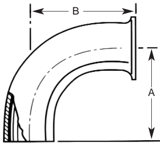
L2CM7 Elbow - Weld x Clamp Standard 90'
