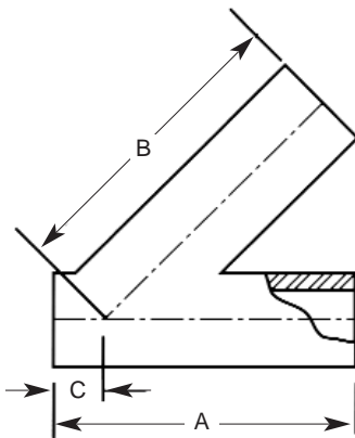
L28A-7 "Y" - Lateral Y Weld Style
