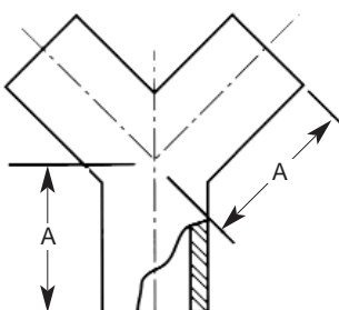
L28B-7 "Y" - True Y Weld Style
