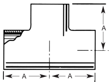
L7WWW7 Tee- Weld Short
